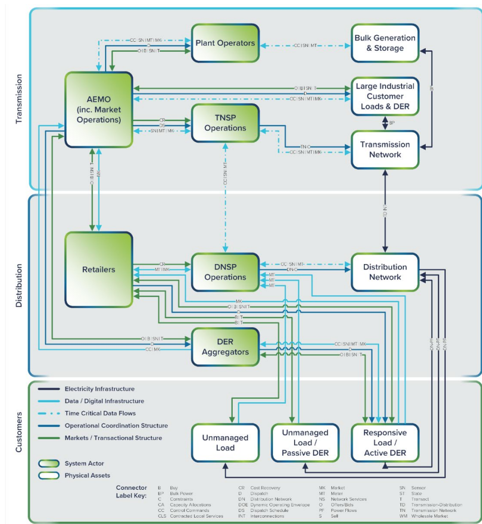
Figure 23: The as-built structural arrangements of the NEM were originally configured to enable the top-down management of a unidirectional power system [1]
