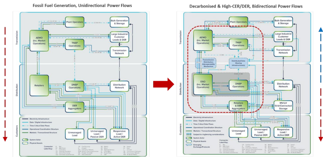
Figure 44: One credible view of how the NEM's legacy structures will need to change to enable high-CER/DER futures similar to AEMO's Step Change scenario [134]
