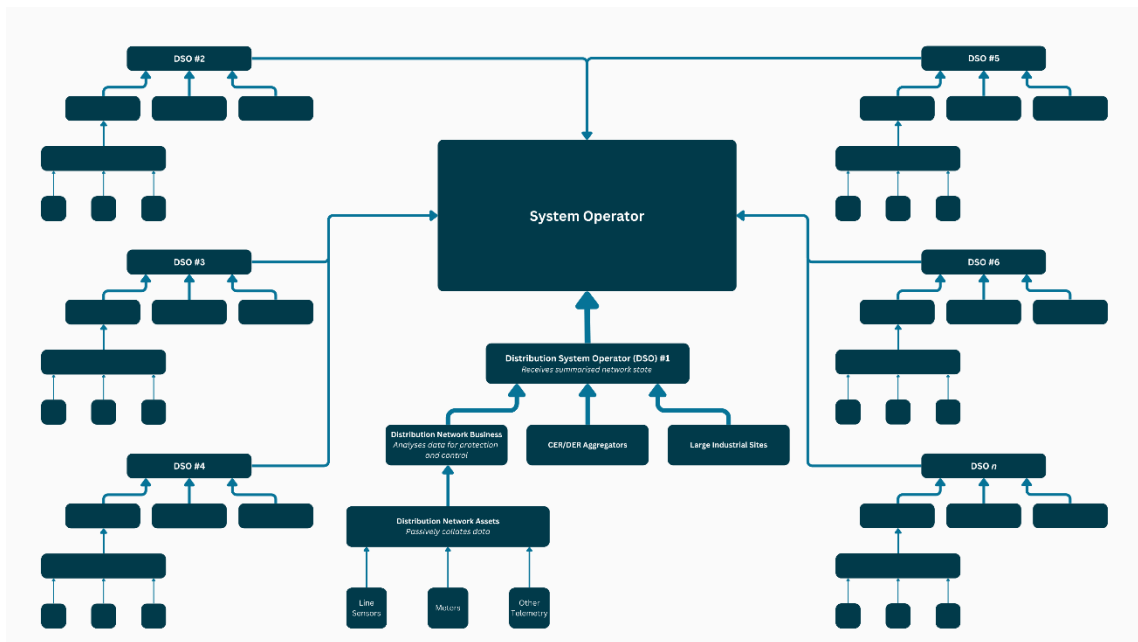
Figure 42: Dataflows viewed from a whole-system perspective, highlighting the critical need for established data transformation approaches
